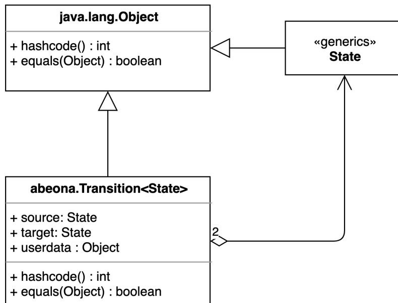
Figure 4.3: The UML diagram specifying the representations for states and transitions.
