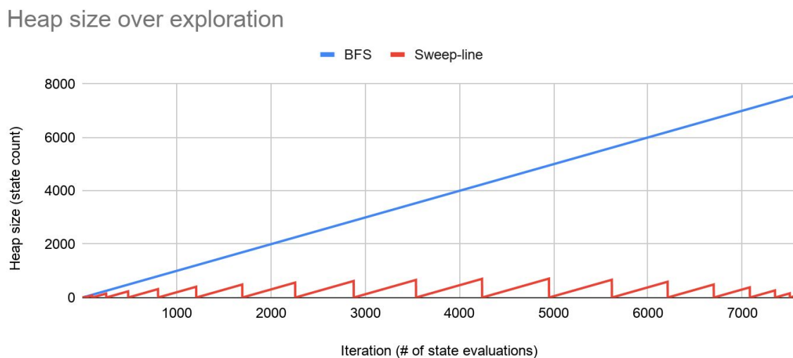
Figure 5.15: The difference between sweep-line and BFS approaches.
