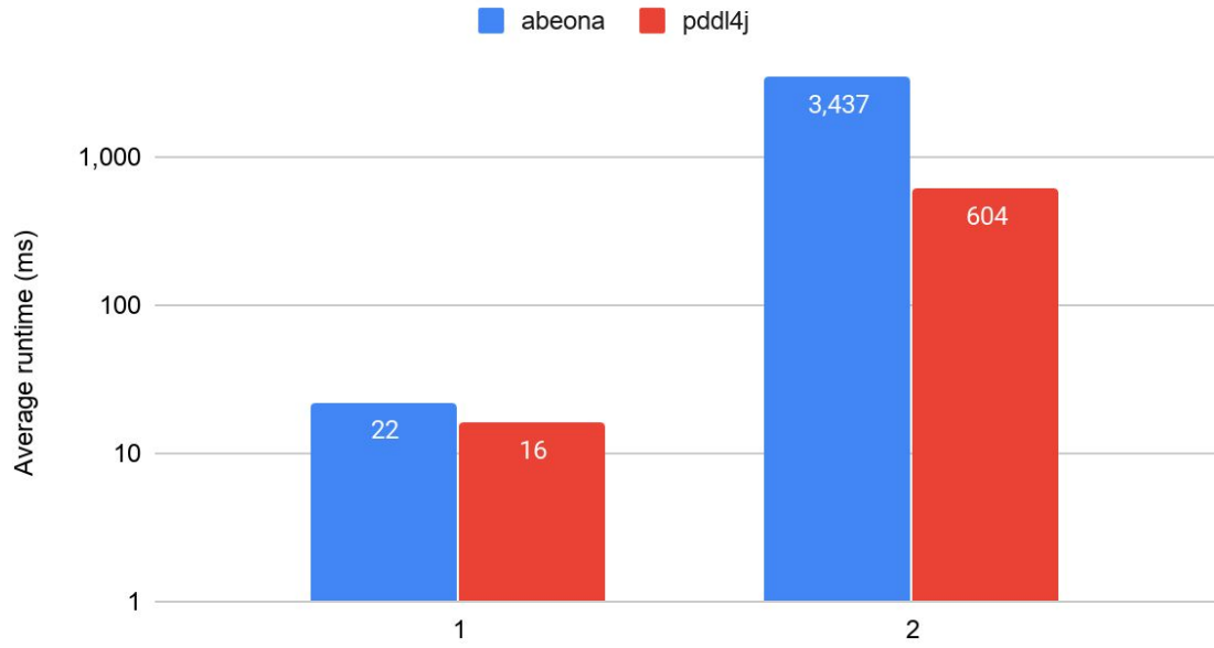
Figure 5.8-C: The runtime results for BFS implementations on depots problems
